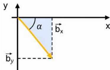
Figura 1.20: Componentes rectangulares del vector |\vec{b}| = 4 , \alpha = -50^\circ .
