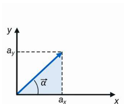
Figura 1.19: Componentes rectangulares del vector |\vec{a}| = 3, \alpha = 45^\circ .
